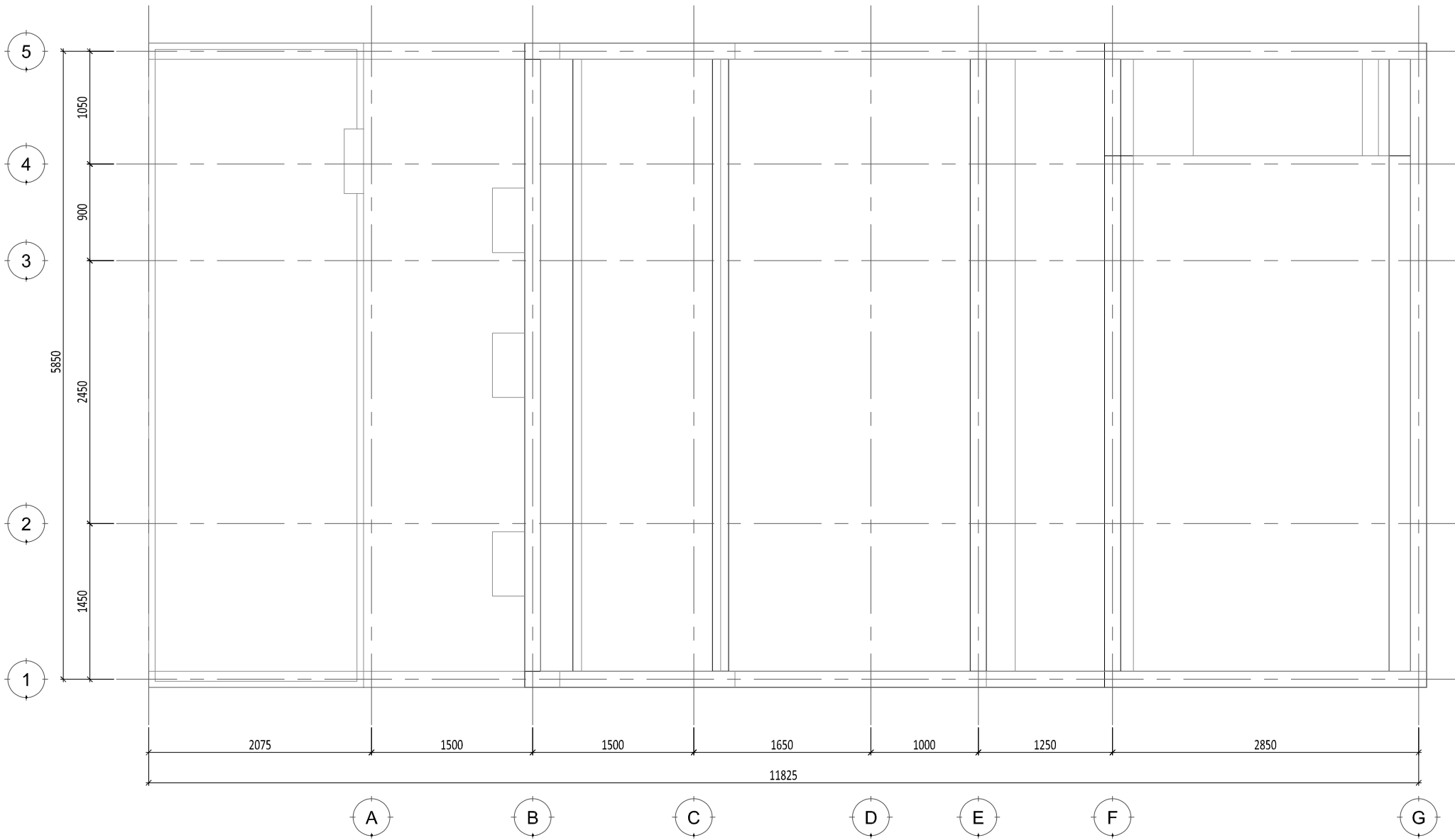
1 DENAH ATAP SCALE 1 : 50 (A4)
