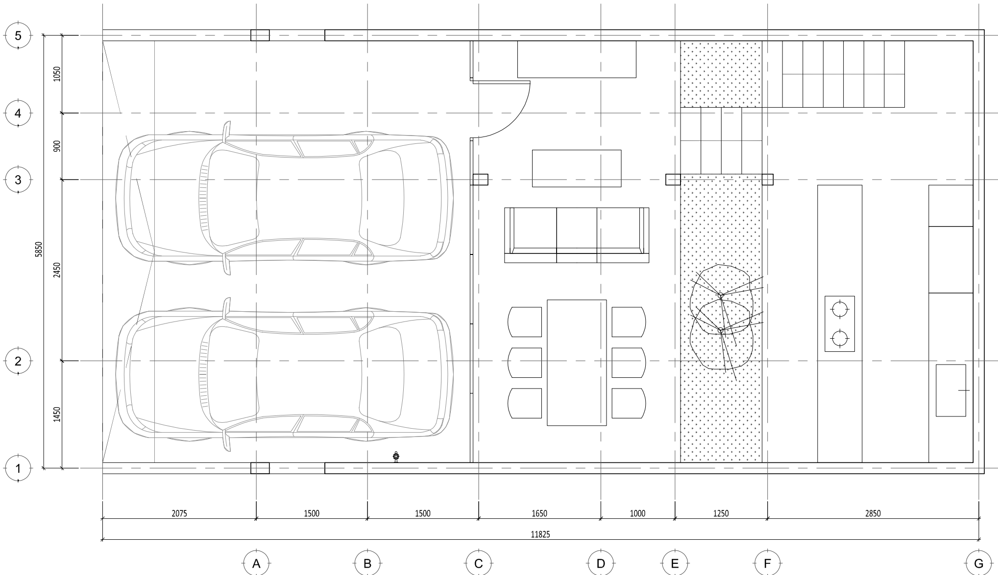
1 DENAH LANTAI 1 SCALE 1: 50 (A4)
