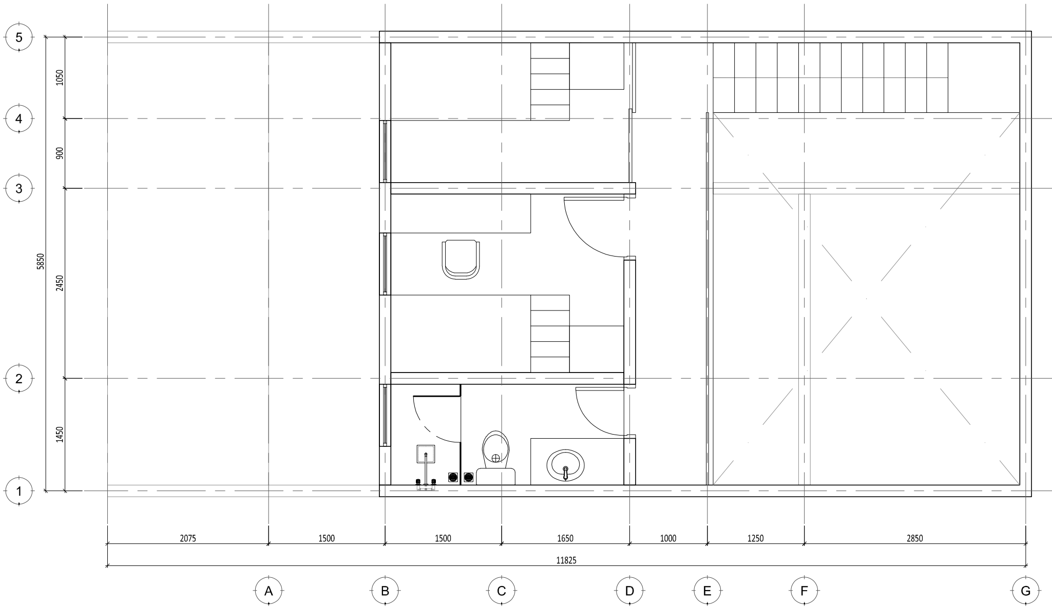
1 DENAH LANTAI 3 SCALE 1: 50 (A4)
