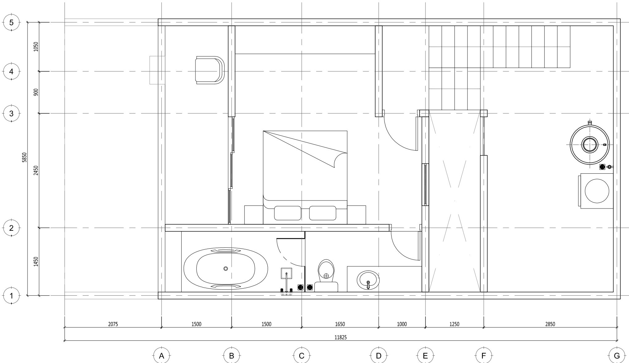
1 DENAH LANTAI 2 SCALE 1: 50 (A4)
